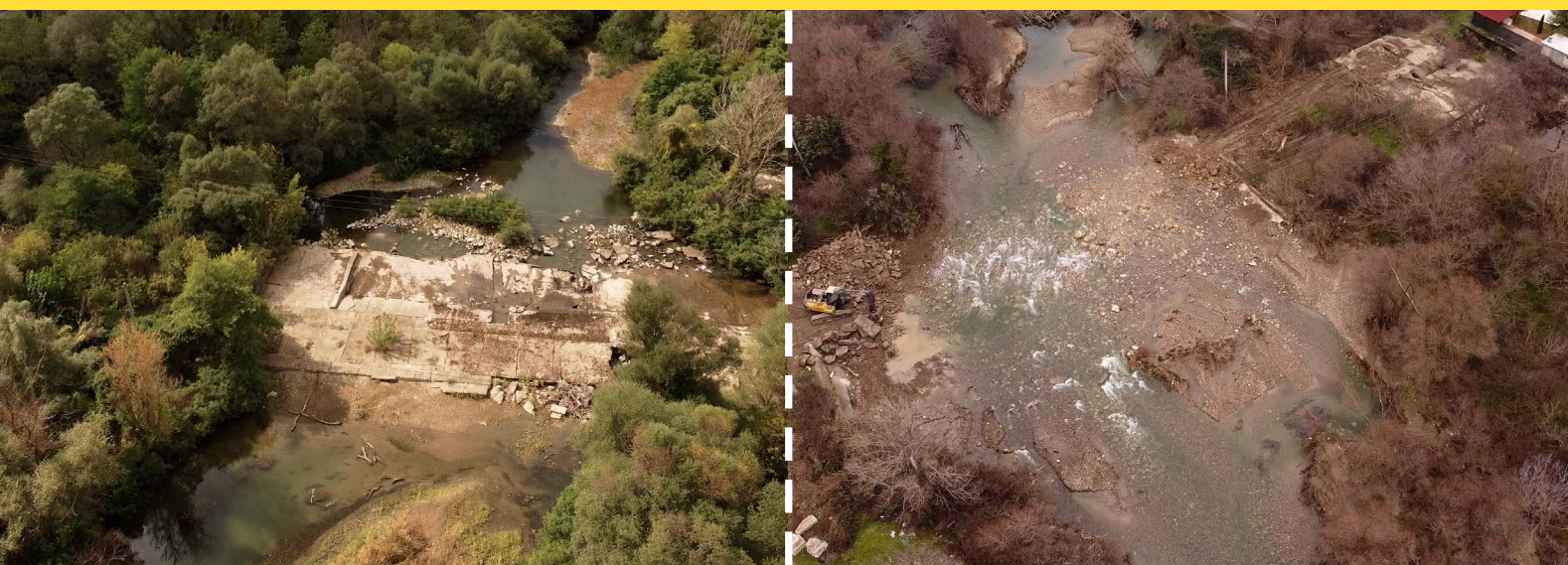
Figure 5. Shuplji Kamen barrier site at Pčinja River in North Macedonia, (left) during and (right) after the removal works © Eko-svest
