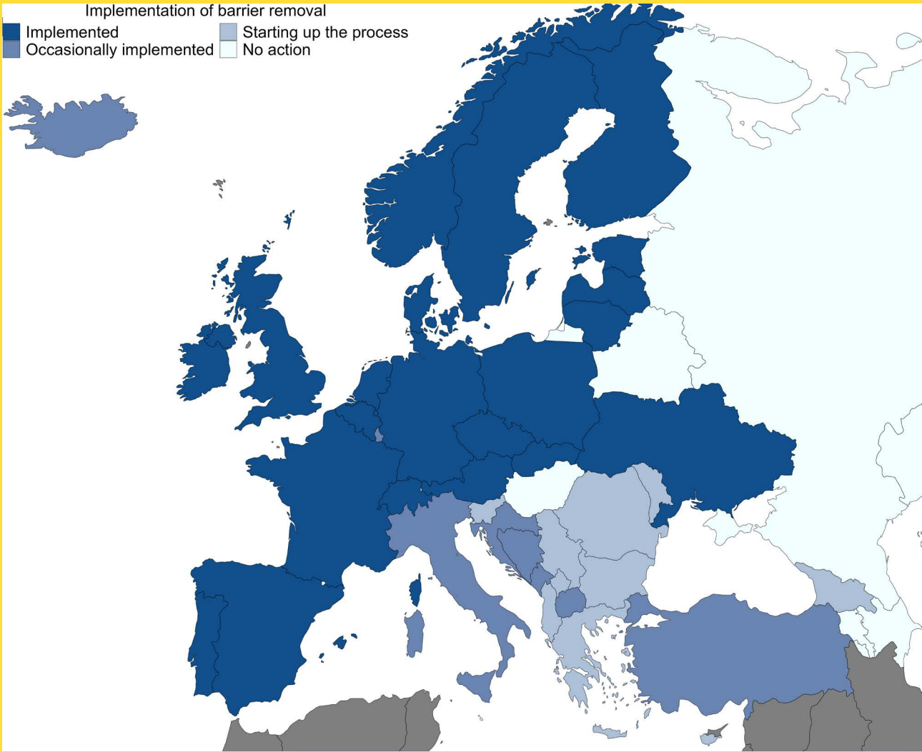
Figure 2. Implementation of barrier removal as a river restoration tool in Europe. Note: barrier removals which took place in England, Scotland, Wales and Northern Ireland are considered under the UK as a single unit; Implemented = barrier removals occurred at least in three of the last five years; Occasionally implemented = barrier removals occurred in one or two years in the last five years; Starting up the process = actions that will lead to future barrier removals have taken place; No action = no actions relevant to barrier removal known to DRE
